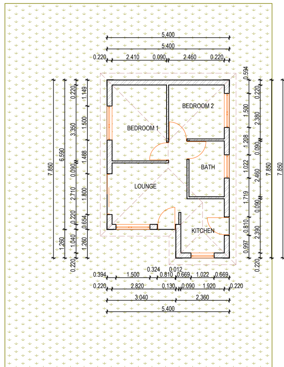
0. Ground Floor 1:100
