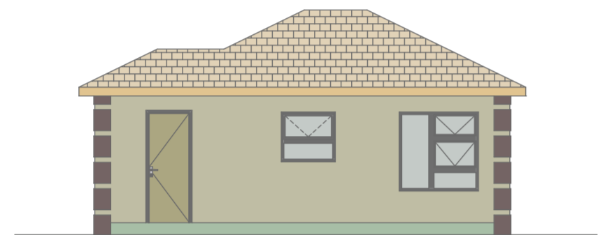
East Elevation 1:100
