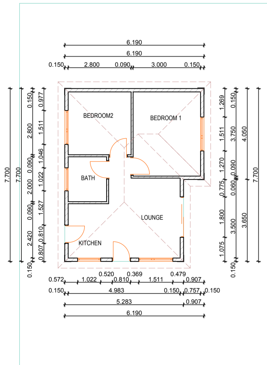
0. Ground Floor 1:100
